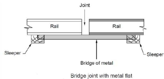
Bridge joint with metal flat
