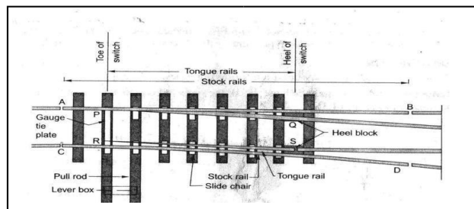
FIGURE: DETAILS OF SWITCH
