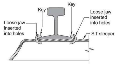
Sleeper with loose jaws inserted into holes
