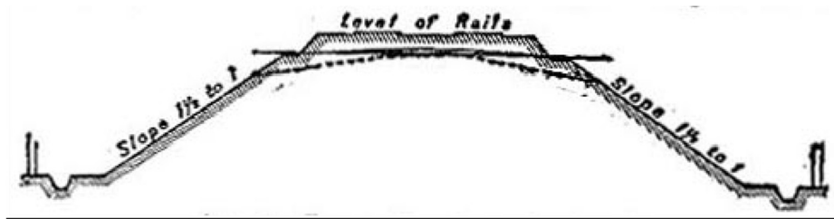
Typical Section of Railway in embankment.
