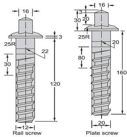
Screw spikes
