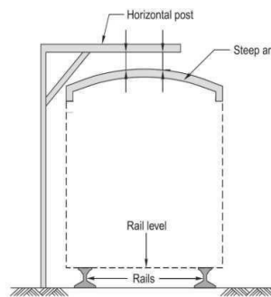
Fig. 2.2 Loading gauge
