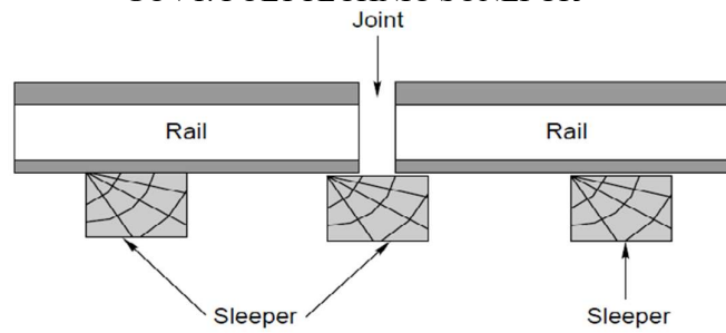
Supported rail joint
