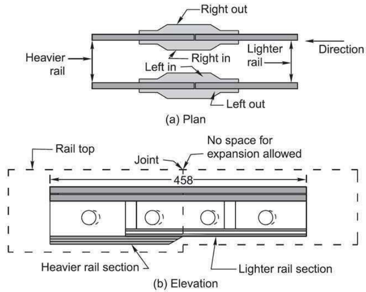
Combination fish plate (dimensions in mm)
