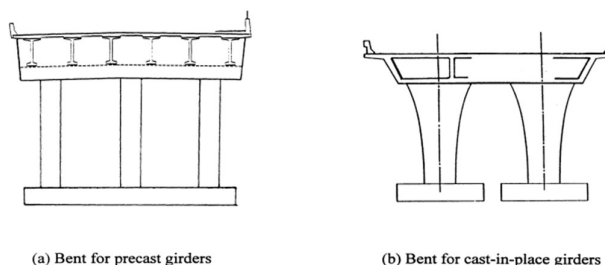
(a) Bent for precast girders
