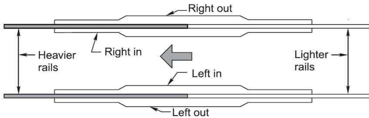
Marking of combination fish plates
